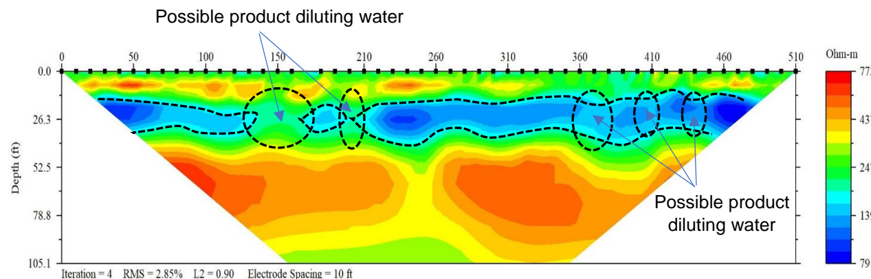
Figure 2. The above image is an example of an electrical resistivity cross section from the project. Such an ER survey permits characterization of subsurface features and designates possible locations of the diesel (product) spill plume.
